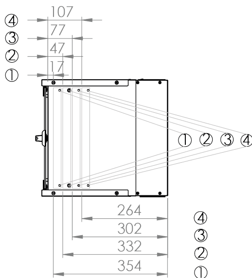
19" cabinet in the top view
